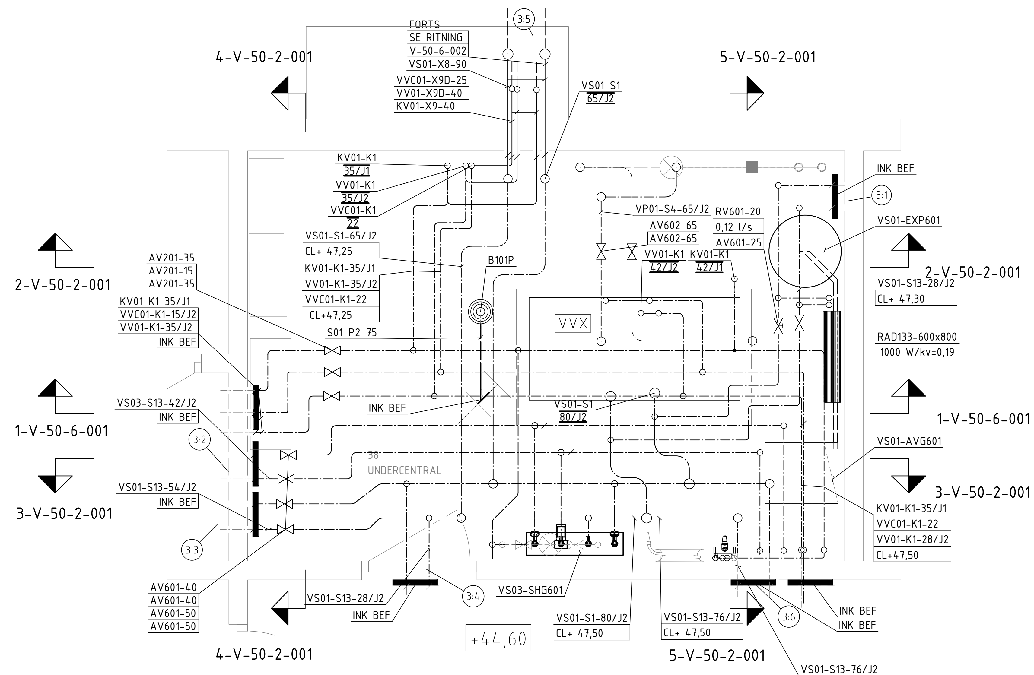
DELPLAN UNDERCENTRAL SKALA 1:20
